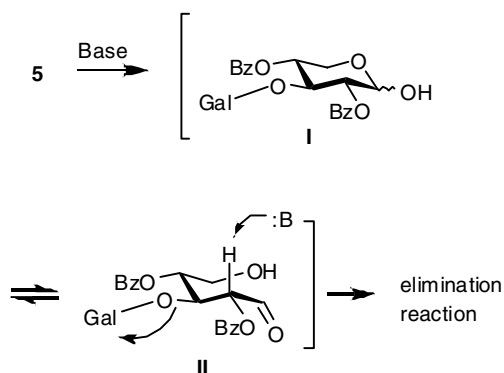
Scheme 2. Proposed mechanism for the cleavage of the glycosidic bond during the debenzylation of 5 .
