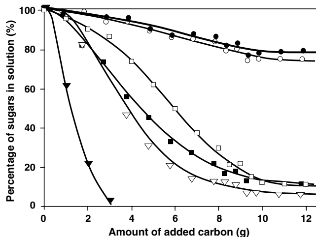
Figure 1. Percentage of remaining sugars in solution after addition of activated carbon to the reaction mixture: ●, D-xylose; ○, D-galactose; ■, 1 ; □, 2 ; ▽, 3 ; ▼, 6 .
