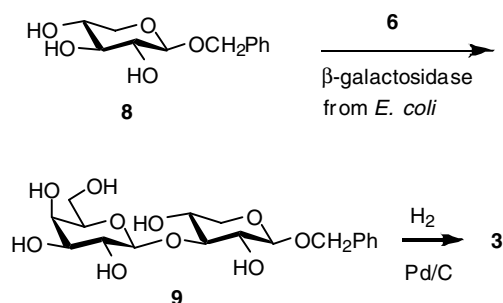
Scheme 3. Synthetic pathway for disaccharide 3 .
