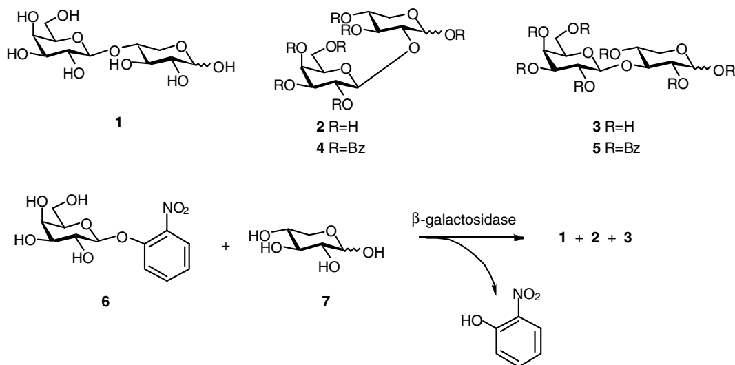
Scheme 1. Synthesis of disaccharides 1 , 2 , and 3 by galactosidation of D-xylose ( 7 ) using a \beta -galactosidase.
